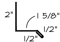
Header Trim
